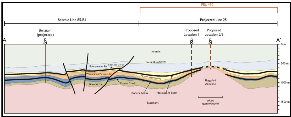
Figure 2 - PEL 470 schematic cross-section. For illustration only, drilling will test formations.
