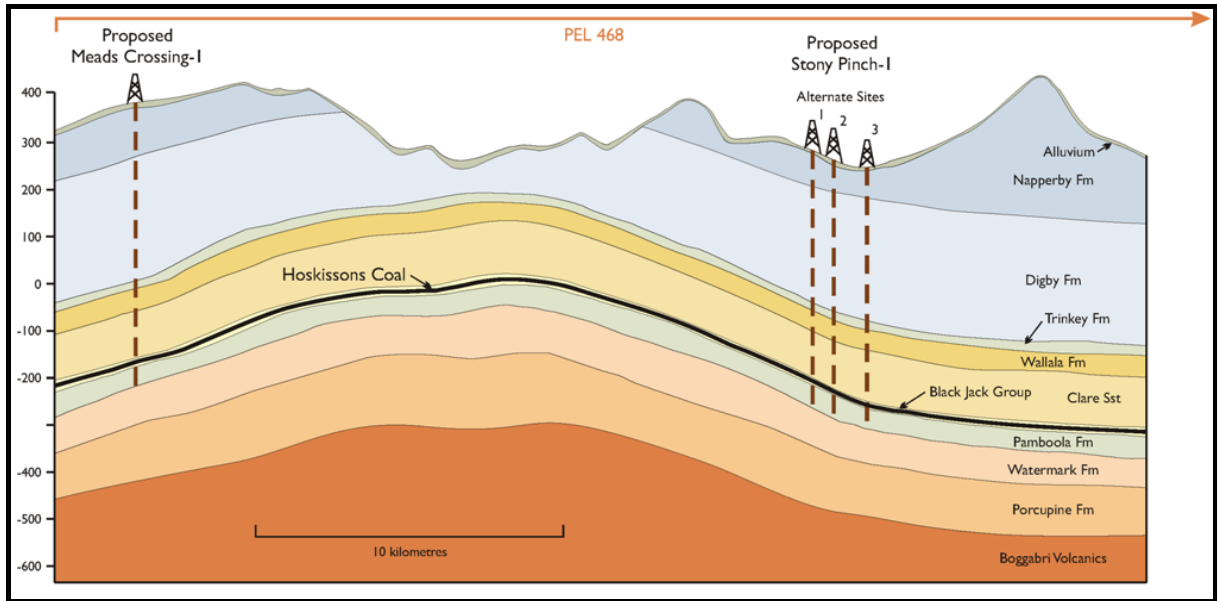
Figure 1 - PEL 468 schematic cross-section. For illustration only, drilling will test formations.
